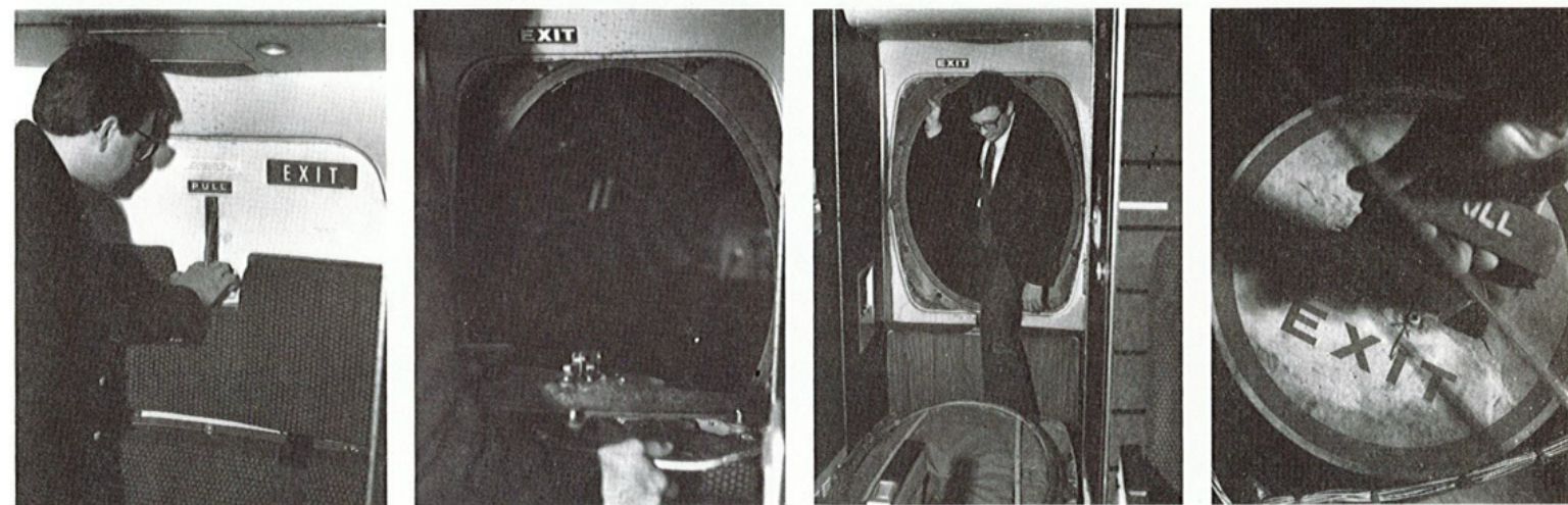
Located at the rear of the aircraft is either a plug hatch type or a pressure bulkhead door. Located in tailcone area.
